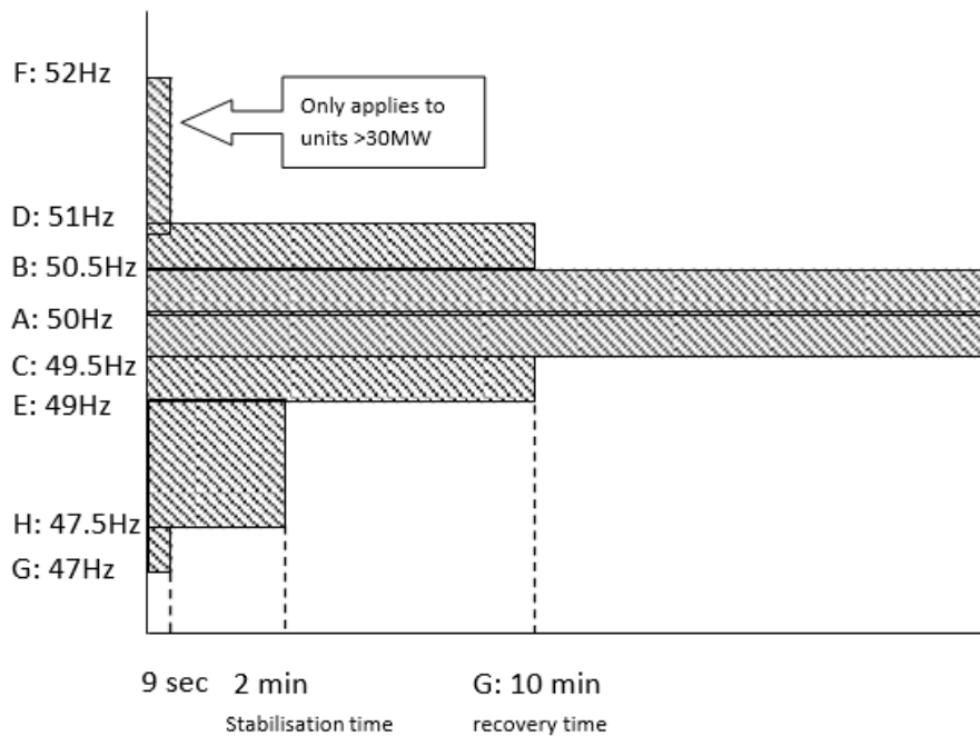
FIGURE 3. FREQUENCY DISTURBANCE RESPONSE MINIMUM ACCESS STANDARD DSDA
