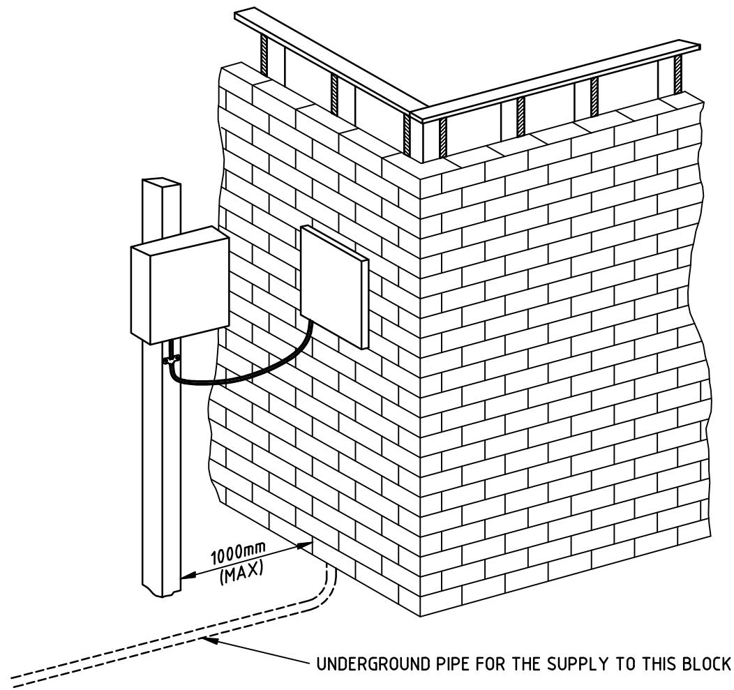
OPTION 1 TEMPORARY OVERHEAD CONSUMER SERVICE MAINS
