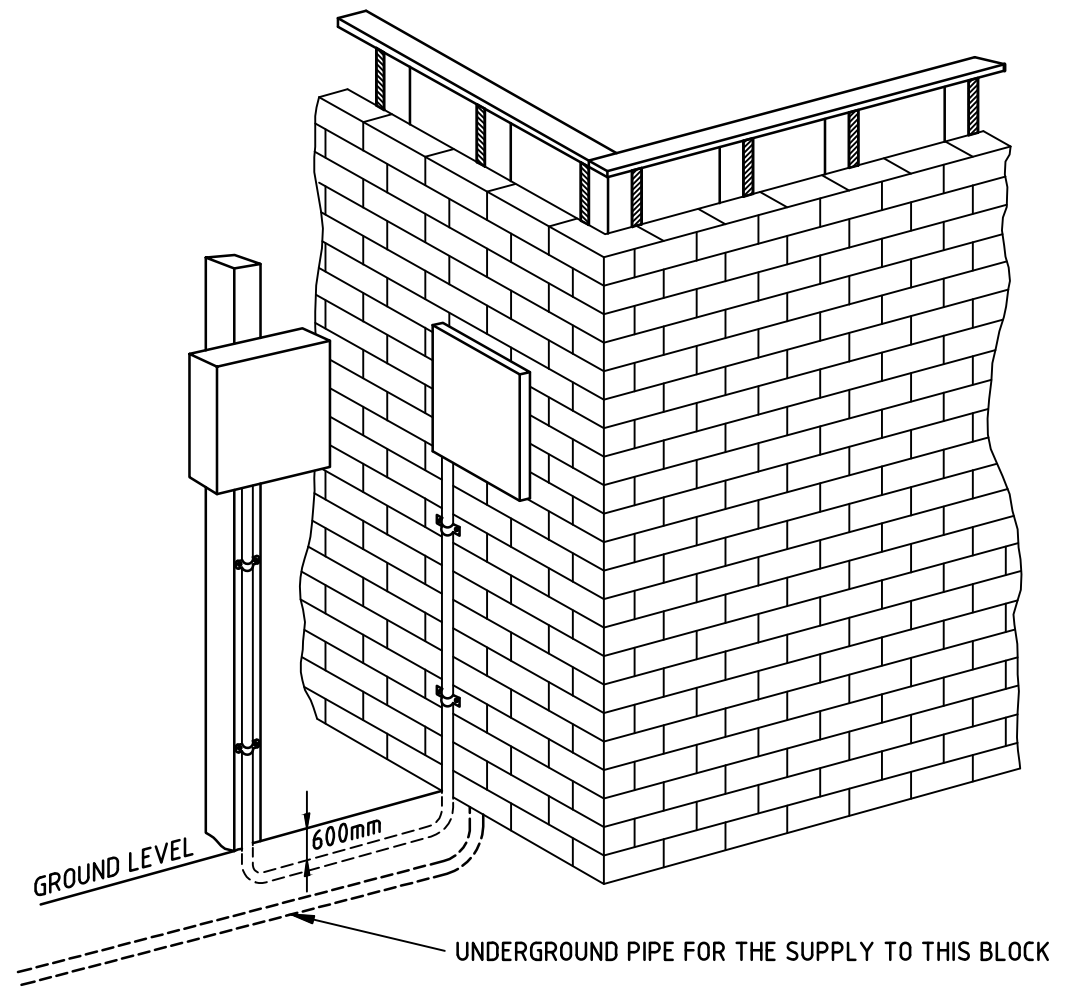
OPTION 2 TEMPORARY UNDERGROUND CONSUMER SERVICE MAINS
